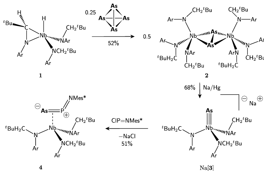
Figure 1. Three-step synthesis of the \eta^2\text{-AsPNMes}^* complex 4 in a sequence encompassing \text{As}_4 activation, \mu\text{-As}_2 ligand reductive cleavage, and terminal arsenide functionalization with the [\text{PNMes}^*]^+ electrophile.
