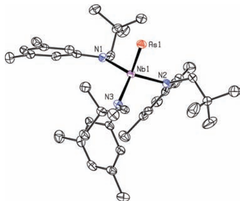
Figure 2. Molecular structure of anion 3 as found in crystals of the salt [\text{Na}(12\text{-crown-}4)_2][\text{As}=\text{Nb}(\text{N}[\text{Np}]\text{Ar})_3] shown with 50% probability thermal ellipsoids. Selected interatomic distances ( \text{\AA} ) and angles (deg): Nb1–As1, 2.3078(5); Nb1–N1, 2.107(2); Nb1–N2, 2.058(2); Nb1–N3, 2.051(2); As1–Nb1–N1, 108.10(7); As1–Nb1–N2, 103.48(7); As1–Nb1–N3, 100.89(7).
