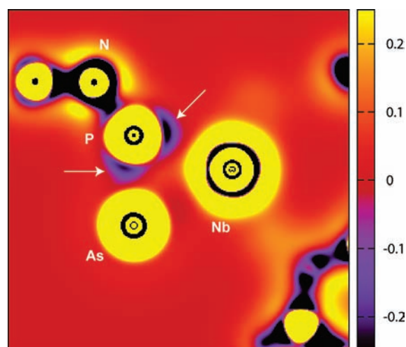
Figure 4. Plot of the Laplacian of the electron density in units of e/a_0^3 for the model system of 4 , (\eta^2\text{-AsPNMe}_s^*)\text{Nb}(\text{N}[\text{Me}]\text{Ph})_3 ; the plot is in a plane defined by the Nb, As, and P nuclei. Two small arrows indicate areas of valence-shell charge concentration in the P–Nb and P–As bonding regions.
