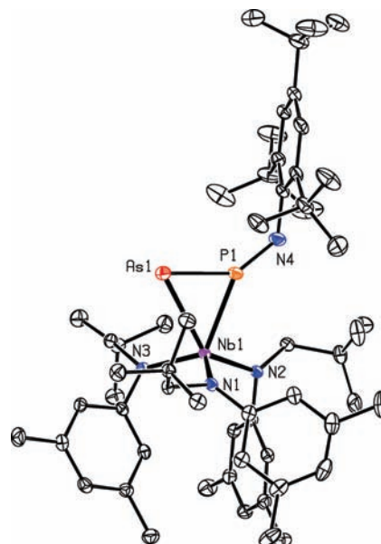
Figure 3. Molecular structure of complex 4 shown with 50% probability thermal ellipsoids. Selected interatomic distances ( \text{\AA} ) and angles (deg): As1–P1, 2.1296(6); P1–N4, 1.564(2); Nb1–As1, 2.6704(3); Nb1–P1, 2.4799(6); As1–P1–N4, 140.56(8); As1–P1–Nb1, 70.335(19); Nb1–As1–P1, 60.989(17).
